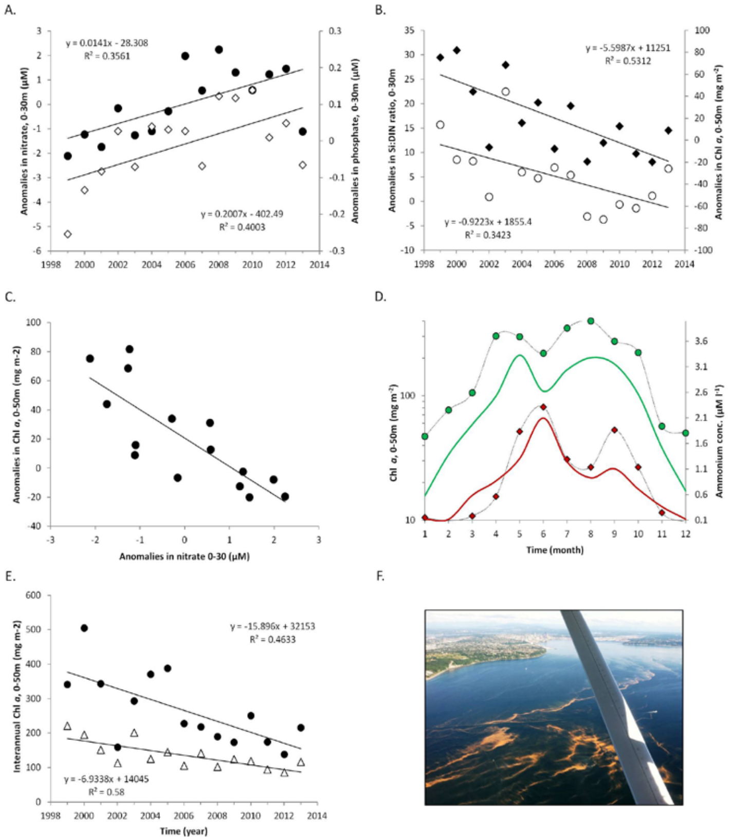
Figure 16. Puget Sound-wide annual anomalies of (A) nitrate (black circles) and phosphate (white diamond), (B) the ratio of Si:DIN (white circles) and chlorophyll-a (black diamond) over the period from 1999-2013. Correlation of Puget Sound-wide long-term anomalies for nitrate and Chl a (C). (D) Puget Sound-wide seasonality and temporal coupling between Chl a (green circles) and ammonium (red circles) for 2013, and time averaged for the years 1999-2012 (green line, Chl a; red line, ammonium). (E) Long-term trends in Puget Sound wide average phytoplankton biomass, for yearly average (triangles) and averages specific to the period July-December, highlighting a preferred decline in late summer. (F) Example of the end of strong Noctiluca bloom surfacing in Central Basin in 2013.
