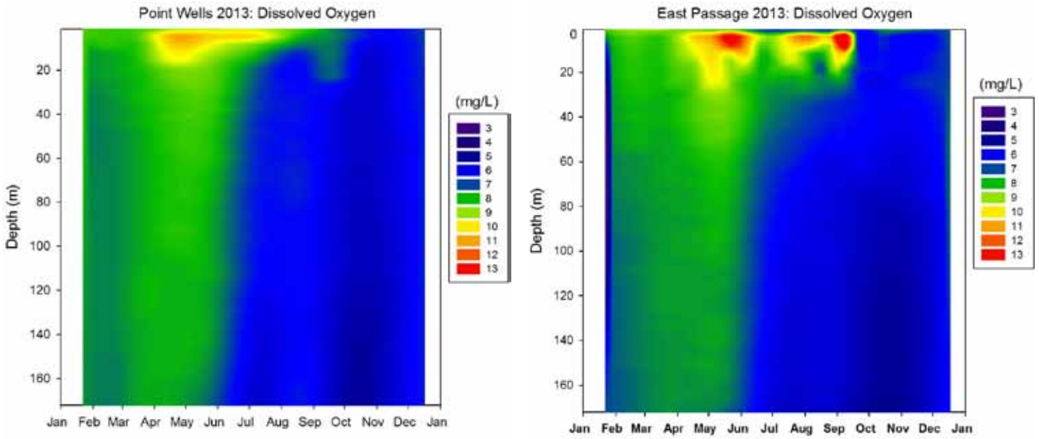
Figure 23. 2013 dissolved oxygen levels at two sites in the Central Basin. An increase in oxygen from phytoplankton blooms is evident, particularly in East Passage.
