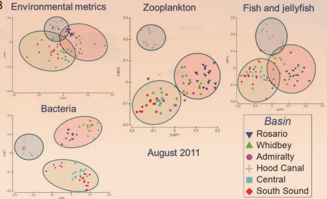
Figure 35. (next page) A. Seasonal trends for dissolved inorganic nutrients (nitrogen in black and phosphate in blue) and microbial indicators (chlorophyll- a in green and heterotrophic production in purple) for all sites in Puget Sound (upper graphs) and by sub-basins (lower graphs) in 2011. Plots are best regressions \pm 95% confidence intervals. B. Multivariate analysis of sub-basin differences in environmental metrics, bacterial diversity, zooplankton taxa, and fish and jellyfish species captured in August 2011. Canonical analysis of principal coordinates explores the hypothesis of sub-basin differences by maximizing basin differences in observations (each point is a sampling site) and mapping them in two unitless axes.
