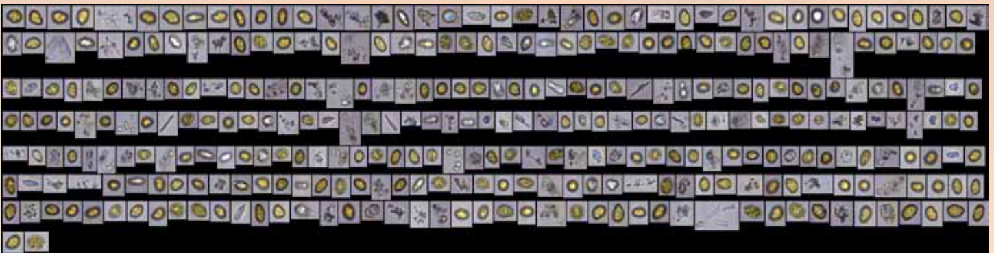
Figure 31. Composite of FlowCam images for the 12-17 mm ABD (area based diameter) size fraction of the Dockton sample that was collected July 17 (L58254-5 at MSWH01, not in LIMS). Heterosigma cells dominate the size fraction.
