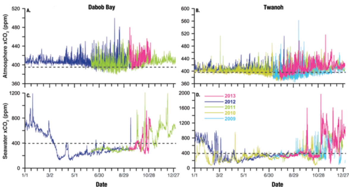
Figure 20. The mole fraction of carbon dioxide (xCO 2 ) in air at 1.5 m above seawater (A, B) and surface seawater at 0.5 m depth (C, D) through the full annual cycle on the surface ORCA moorings at Dabob Bay and Twanoh. Data from all deployment years are included for comparison (color key in panel D applies to all panels). Approximate 2013 global average atmospheric xCO 2 of 395 ppm is indicated with a dashed line in each panel. Data shown for 2013 at Dabob and for 2009–2012 at Twanoh have not been subjected to quality control, but typical uncertainty associated with xCO 2 measurements from these systems is <2 ppm in the range of 100–600 ppm, increases for values between 600 and 1000 ppm, and is not well constrained above 1000 ppm. Note different scales of vertical axes.
