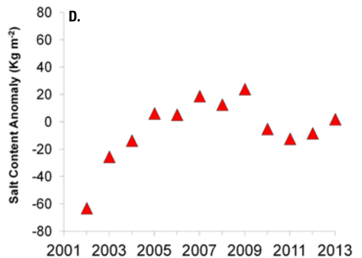
Figure 14. Heat maps of Puget Sound thermal energy (A) and salt content (B) anomalies for the 0-50 m water layer. Anomalies are calculated from site-specific monthly averages using a reference baseline established for 1999-2008. Green = lower, red = higher, black = expected, gray = no data. Puget Sound-wide annual anomalies for (C) temperature and (D) salinity in the 0-50 m water layer from 2002-2013.
