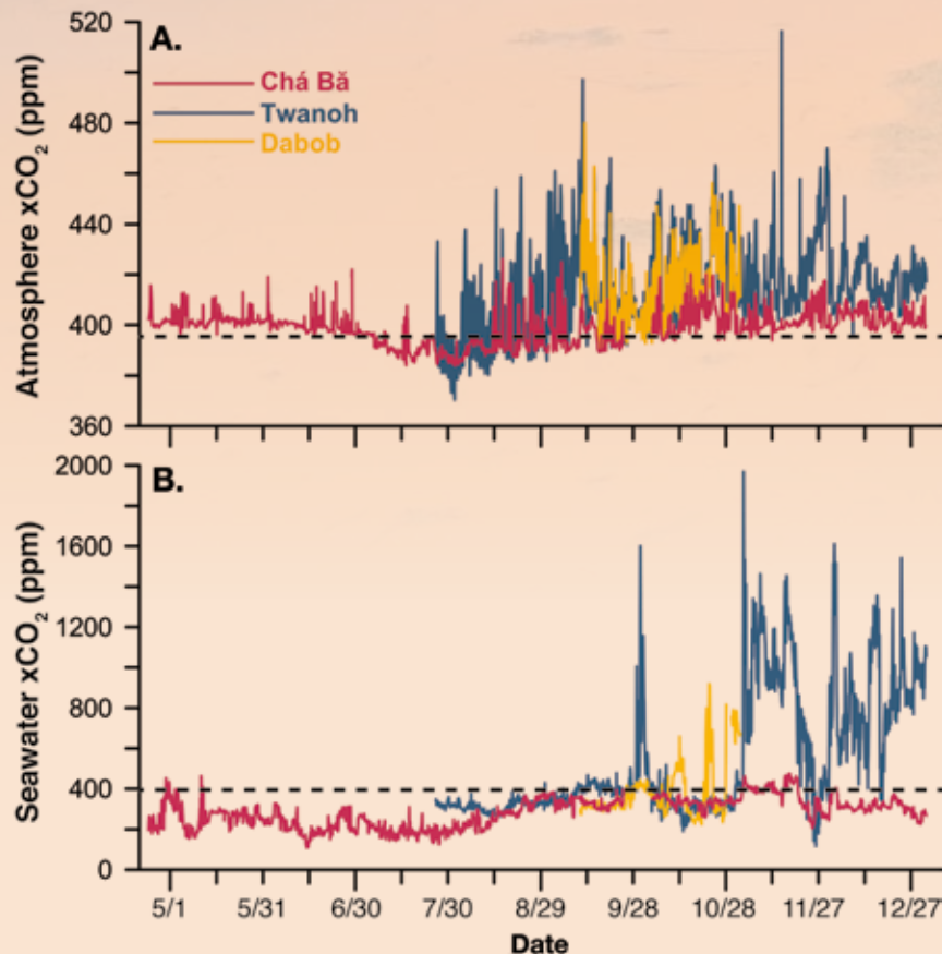
Figure 10. The atmospheric (A) and surface seawater (B) xCO 2 records collected between late April and December 2013 on the Chá bã, Dabob Bay, and Twanoh surface moorings. Information about the layout, axes, and uncertainty associated with this figure is presented in figures 8 and 20.
