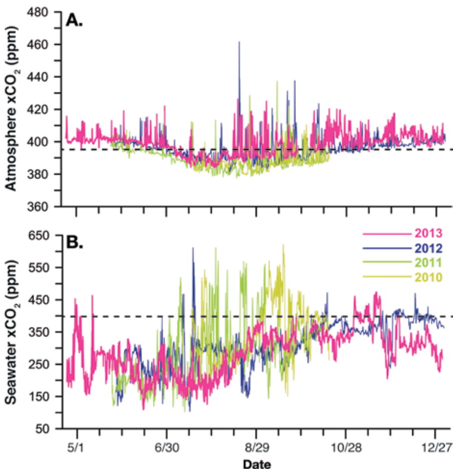
Figure 8. The mole fraction of carbon dioxide (xCO 2 ) in air at 1.5 m above seawater (A) and surface seawater at 0.5 m depth (B) from mid-May through December at the surface Chá bã mooring off La Push, WA. Data from all deployment years are included for comparison (color key in panel B applies to all panels, data available in: Mathis et al. 2011). Approximate 2013 global average atmospheric xCO 2 of 395 ppm is indicated with a dashed line in each panel. Typical uncertainty associated with quality controlled xCO 2 measurements from these systems is <2 ppm for the range 100-600 ppm. Note different scales of vertical axes.
