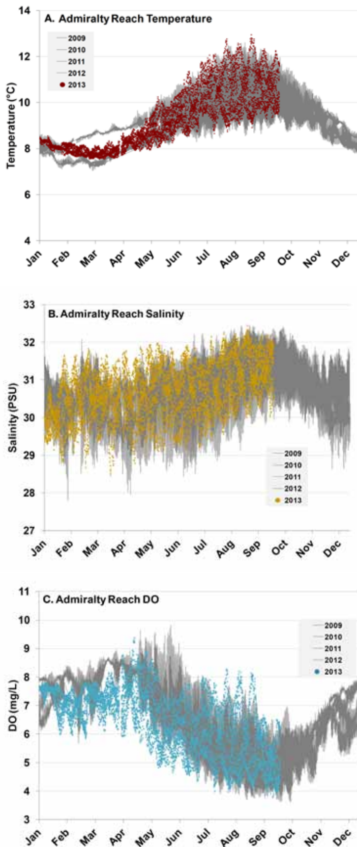
Figure 9. Admiralty Inlet mooring data at ~60 m depth. Shown are continuous measurements collected every 45 minutes of (A) temperature, (B) salinity, and (C) dissolved oxygen.
