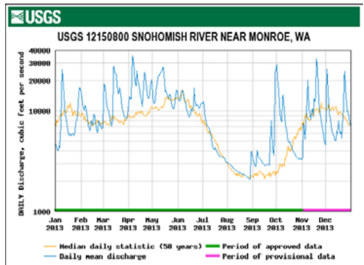
Figure 11. Daily discharge (cfs) at stations in Nooksack, Skagit, Snohomish, Puyallup, Nisqually, and Skokomish Rivers for 2013, compared to long-term median values. Note the period of record varies and is indicated separately for each station.
