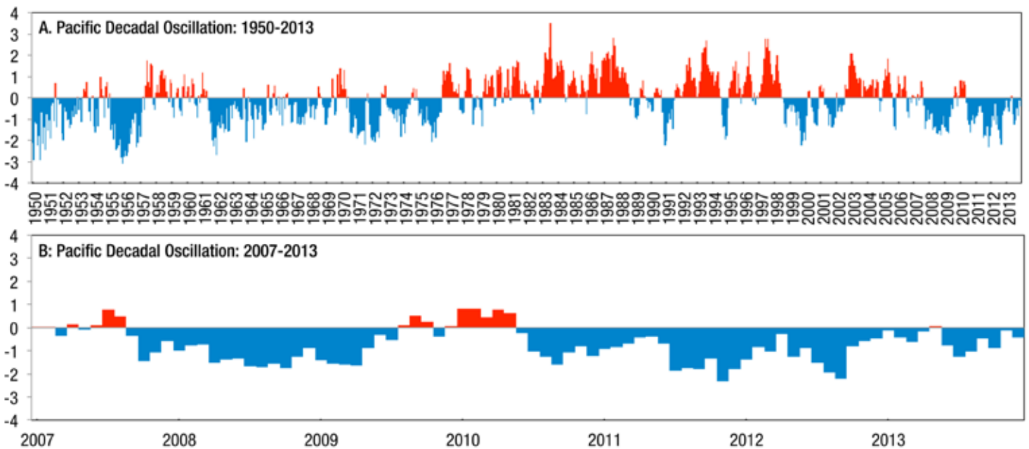
Figure 2. Monthly values of the Pacific Decadal Oscillation index (PDO) from A. 1950-2013 and B. 2007-2013.
