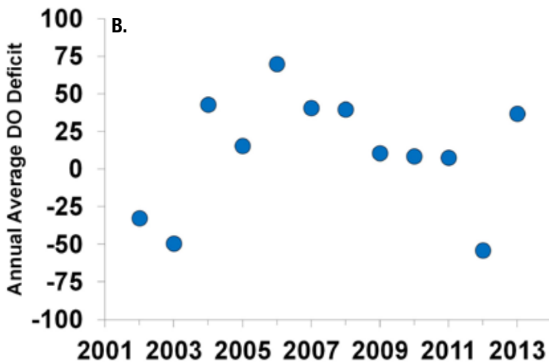
Figure 15. Puget Sound monthly DO deficit anomalies from 2002-2013 for water deeper than 20 m using a reference baseline established from 1999-2008. (A) Heat map of monthly anomalies calculated from site-specific monthly averages. Green=lower, red=higher, black=expected, gray=no data. (B) Puget Sound-wide annual anomaly of the DO deficit from 2002-2013.
