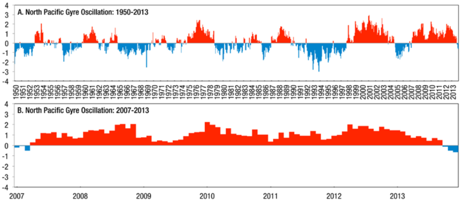
Figure 3. Monthly values of the North Pacific Gyre Oscillation index (NPGO) from A. 1950-2013 and B. 2007-2013.
