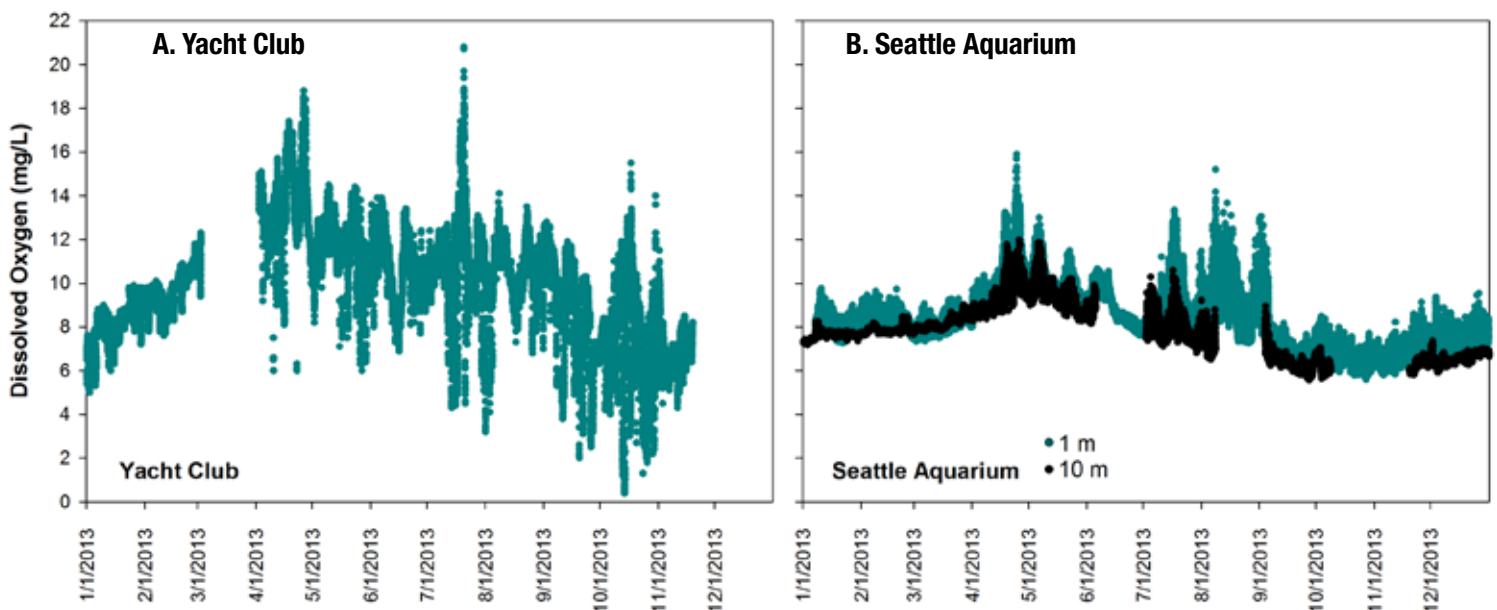
Figure 22. Dissolved oxygen levels in 2013 in inner Quartermaster Harbor (Yacht Club) at 1 m and in Elliott Bay (Seattle Aquarium) recorded every 15-minutes.
