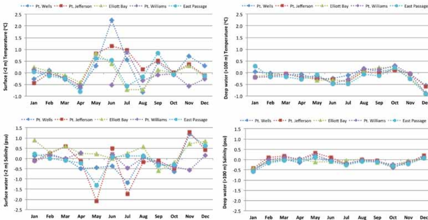
Figure 21. Monthly anomalies of temperature at the (A) surface (<2 m) and (B) depth, and salinity at the (C) surface and (D) depth for five sites in Central Basin in 2013 relative to a long-term average (1999-2010). Negative values indicate colder/fresher water than normal.
