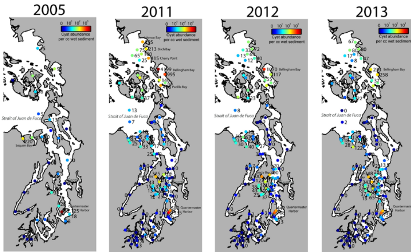
Figure 30. Alexandrium catenella surface sediment cyst distribution maps for winter Puget Sound surveys (number of cysts/cc wet sediment).
