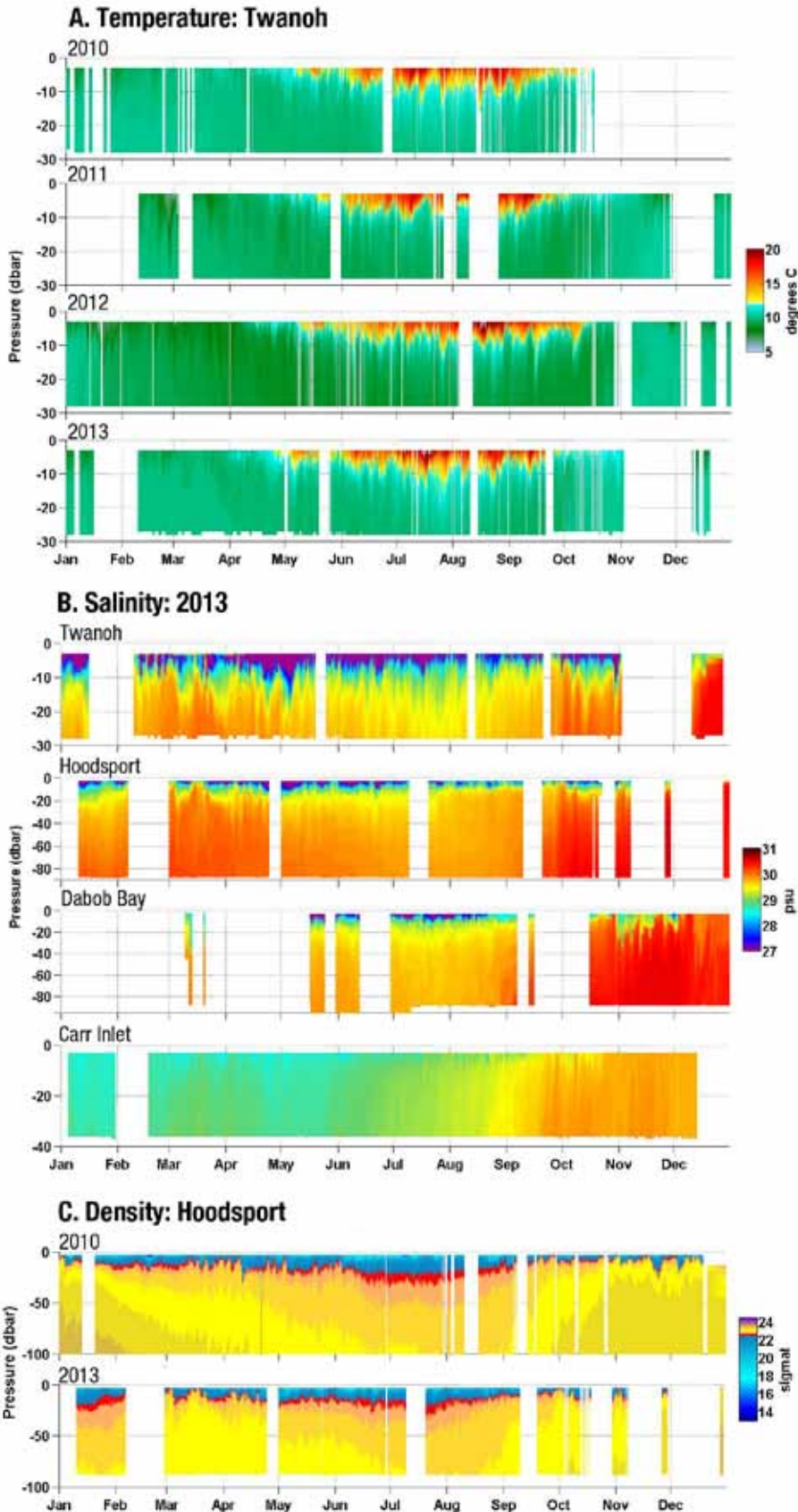
Figure 18. (A) Temperature data at Twanoh (southern Hood Canal) for 2010-2013. Note that pressure in dbars is roughly equivalent to depth in meters. (B) Salinity data from the Twanoh and Hoodsport (southern Hood Canal), Dabob Bay, and Carr Inlet (southern Puget Sound) moorings for 2013. (C) Density ( \sigma_t ) data at Hoodsport (southern Hood Canal) for 2010 and 2013.
