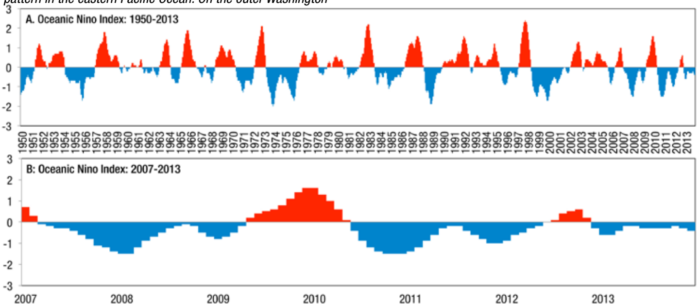
Figure 1. Monthly values of the Oceanic Niño Index (ONI) from A. 1950-2013 and B. 2007-2013.
