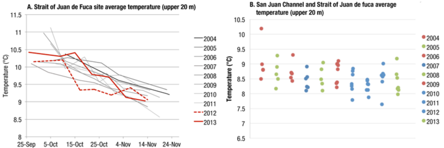
Figure 26. (A) Average seawater temperature during fall in Strait of Juan de Fuca over 10-year time series. (B) Average cruise seawater temperature (both sites) colored by ENSO status (orange = El Niño; blue = La Niña; green = neutral).
