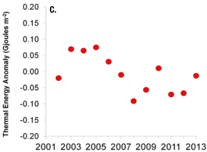
Figure 14. Heat maps of Puget Sound thermal energy (A) and salt content (B) anomalies for the 0-50 m water layer. Anomalies are calculated from site-specific monthly averages using a reference baseline established for 1999-2008. Green = lower, red = higher, black = expected, gray = no data. Puget Sound-wide annual anomalies for (C) temperature and (D) salinity in the 0-50 m water layer from 2002-2013.
