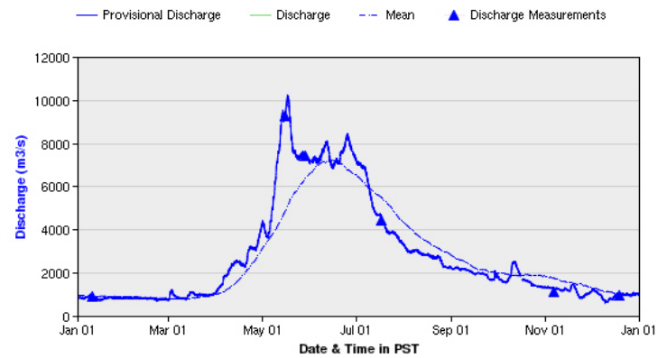
Figure 12. Fraser River daily discharge ( m^3/s ) at Hope, B.C. for 2013, compared to the mean value from long-term records (1912-2014). (Note: 1 m^3/s = 35.3 cfs ).
