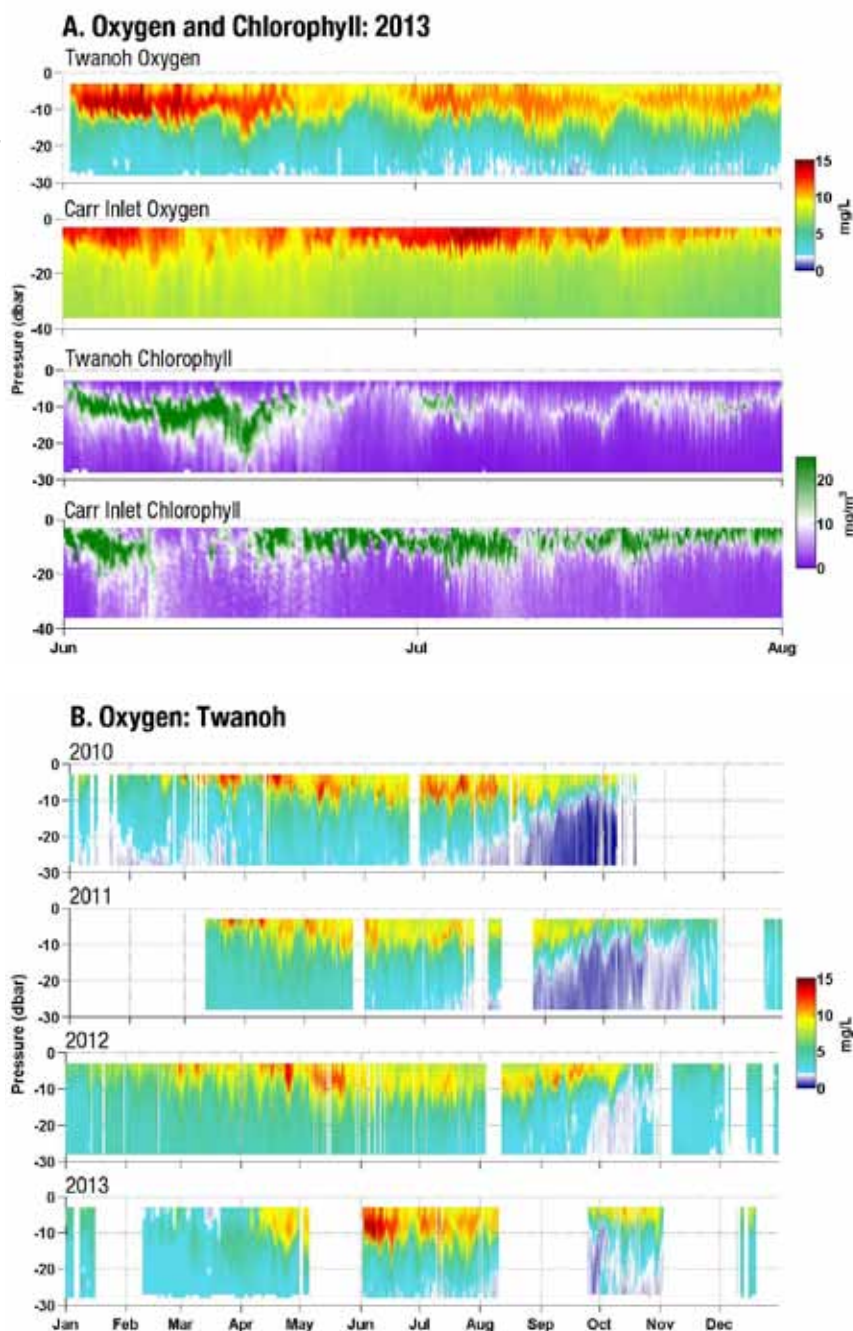
Figure 19. (A) Oxygen (upper two panels) and chlorophyll (lower two panels) concentrations at Twanoh (southern Hood Canal) and Carr Inlet (southern Puget Sound) from June through July, 2013. Note that pressure in dbars is roughly equivalent to depth in meters. (B) Oxygen data at Twanoh (southern Hood Canal) for 2010–2013. Data are colored with a white threshold at 2 mg/L; values below are shaded purple and indicate hypoxic waters.
